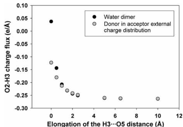
Figure 6. Optimized O 2 –H 3 charge fluxes (in e \text{ \AA}^{-1} ) as a function of the elongation from the MP2/6-31++G(d,p) minimized H 3 ...O 5 distance (in Å) for the SDP-LP/ILP dimer (black circles) and the polarizable LP/ILP electrical model without size donor in the nonpolarizable LP/ILP without size external charge distribution of the acceptor (gray circles). Excluding the H 3 ...O 5 distance, the structures were constrained to the MP2/6-31++G(d,p) optimized dimer structure.
